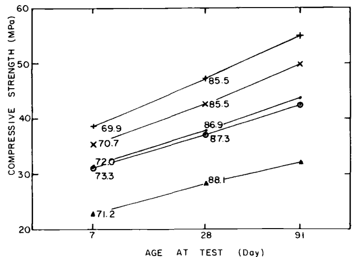
FIG. 1—Age-strength relationship.
