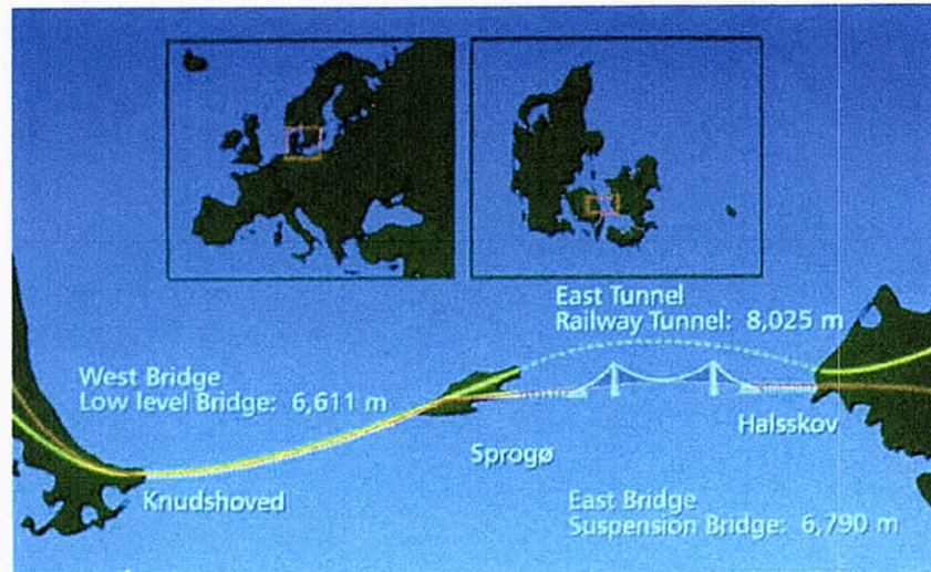
Fig. 1. The Great Belt Link.
