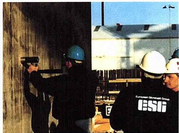
Fig. 7. LOK-test for in-situ strength assessment.
