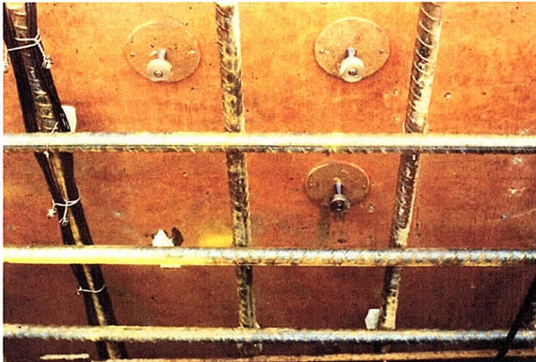
Fig.15. LOK-Test inserts installed in wooden formwork before concrete casting.
