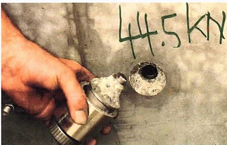
Fig.14. Successfully completed CAPO/LOK-Test of the cover layer of an element.
