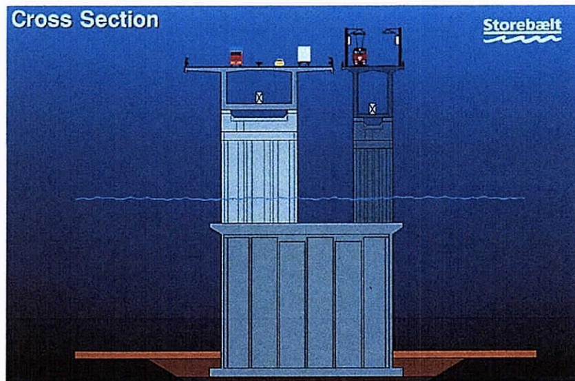
Fig. 3. Cross section of the West Bridge.
