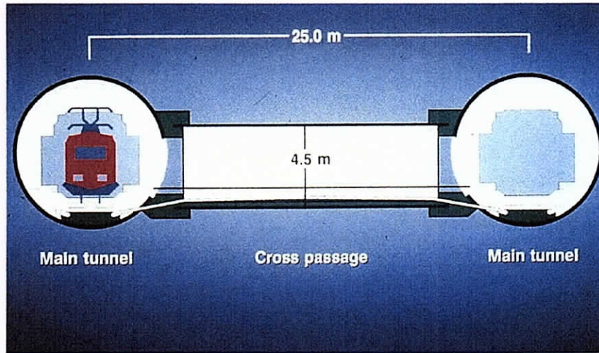
Fig. 2. Cross section of the East Tunnel.
